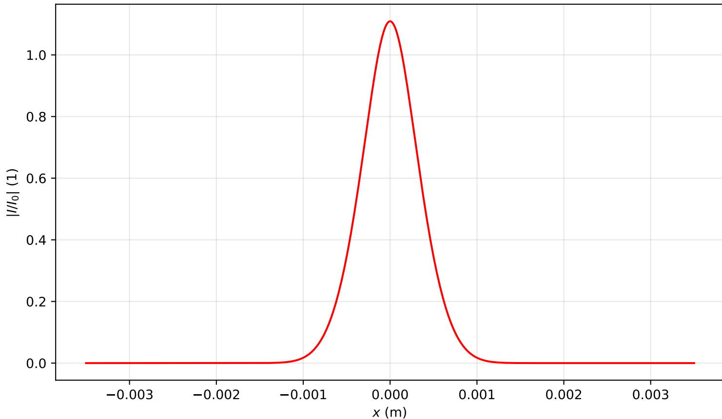
Intensity profile I(x, y = 0, z = 0.239)/I_0 , P_{in}=2.0P_{cr} , artificial time
